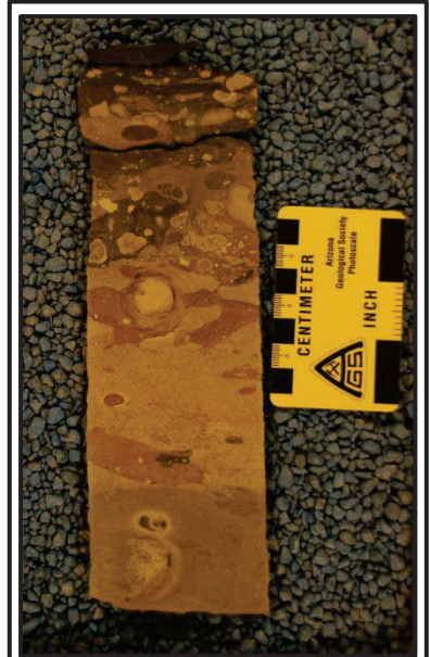
K/Pg boundary from Justiss Oil Company, Inc. LA Central IPNH No. 2 Well-Olla Field LaSalle Parish, Louisiana. From the dark “sliver” at the top, upwards for over 600 ft. the lithology is the Midway Shale.
